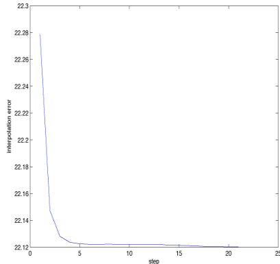
Figure 8: Interpolation of the second example
