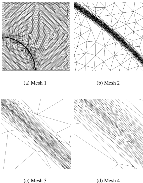
Figure 9: An anisotropic mesh and its details
