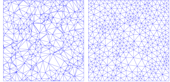
(a) Original mesh (b) Laplacian smoother
